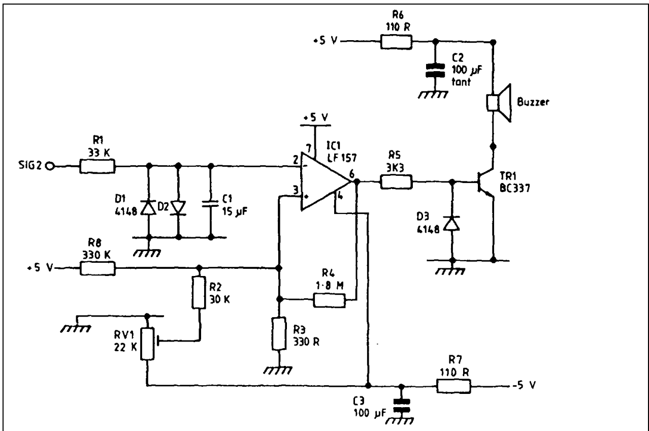
Figure B.2 — Circuit diagram – typical drift alarm unit
