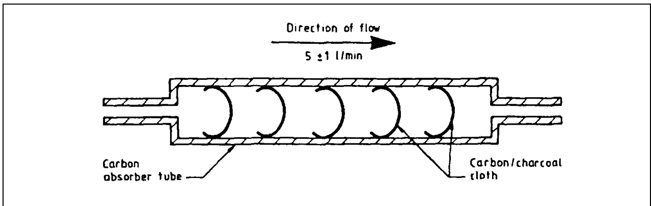
Figure B.1 — Schematic of carbon absorber
