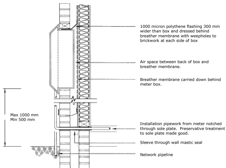
FIGURE 3 - PIPEWORK ROUTE – EXTERNAL
