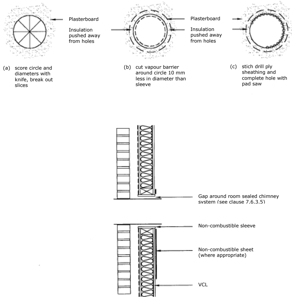
FIGURE 11 - INSTALLATION OF A ROOM SEALED CHIMNEY SYSTEM TERMINAL (CIRCULAR) THROUGH AN EXISTING TIMBER FRAME
