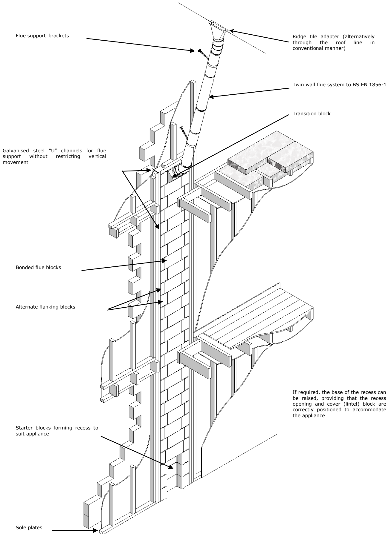
FIGURE 13 - PROPRIETARY PRE-CAST CONCRETE SYSTEM CHIMNEY
