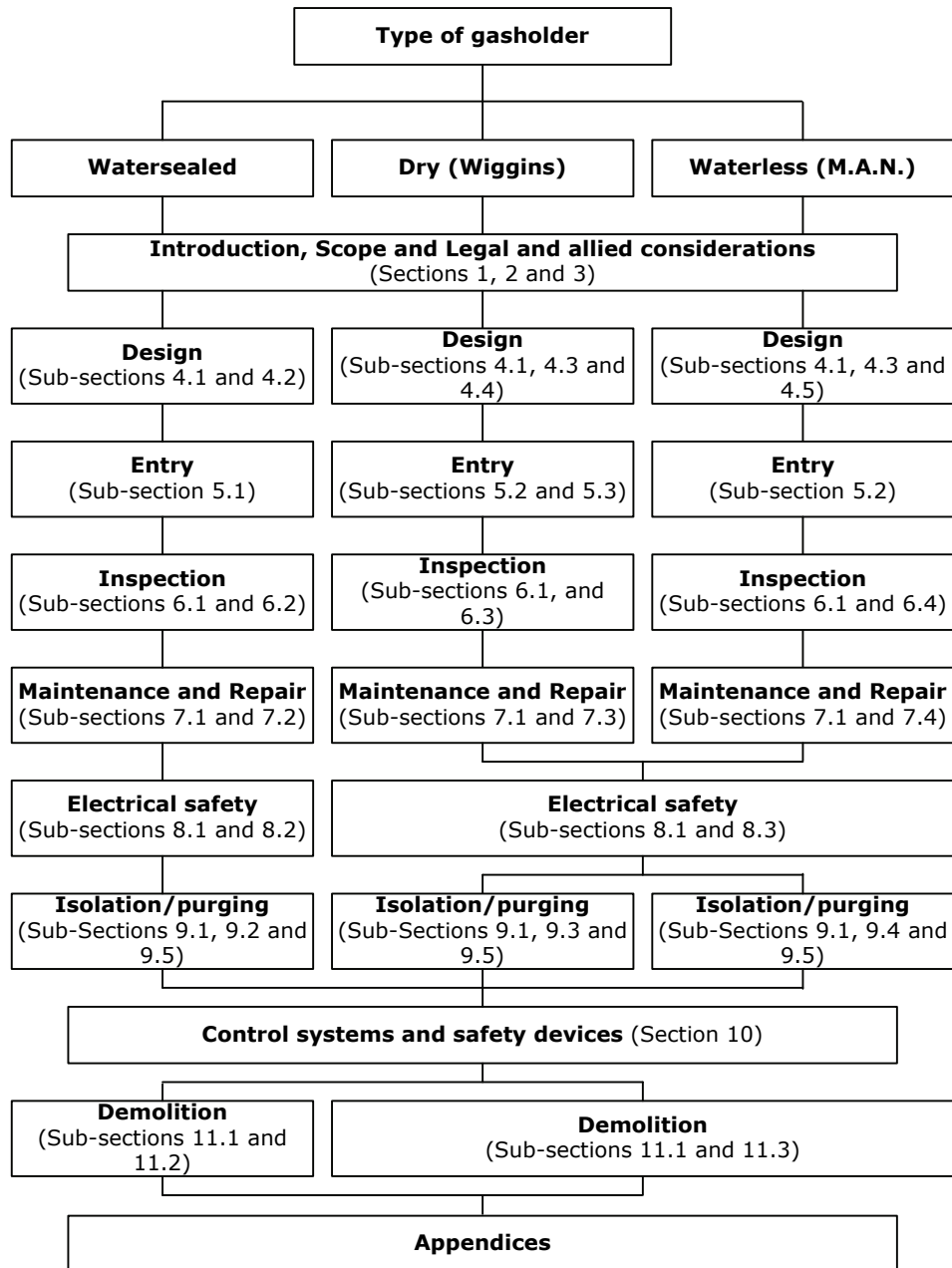
FIGURE 1 - LAYOUT OF IGEM/SR/4
